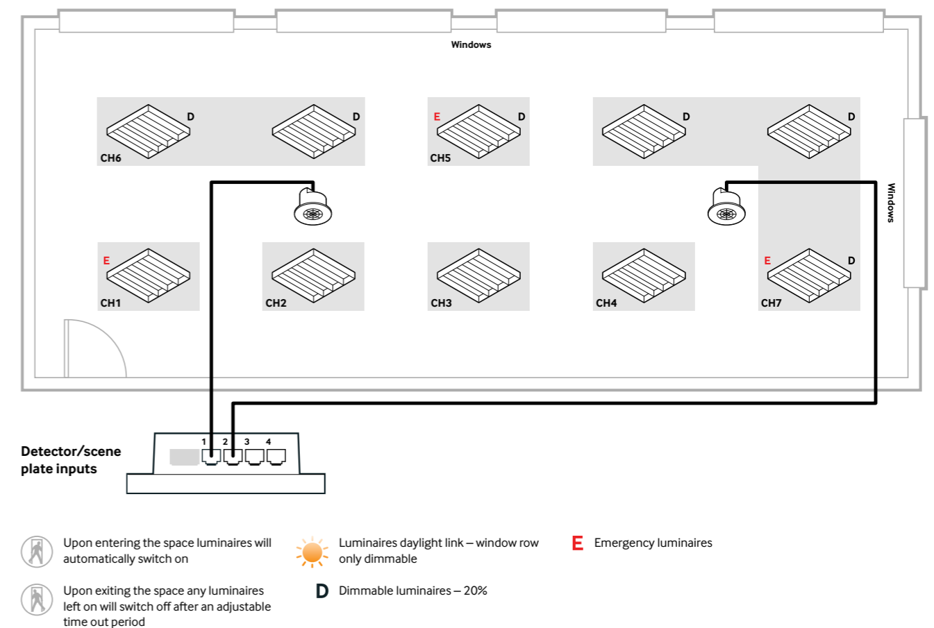
Config 3 – Open plan office working in presence mode with channels 5, 6 and 7 daylight dimming for perimeter row(s).
